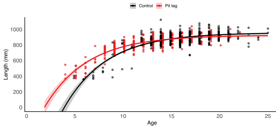
Fig. 3. Length at age data with Pütter-von Bertalanffy curves and 95% confidence intervals in shaded colours, for untagged control eels (black) ( n = 440 ) and PIT-tagged eels released as small yellow eels (red) ( n = 335 ). A minor horizontal jitter was added to the data points to enable better visualization of the data.
