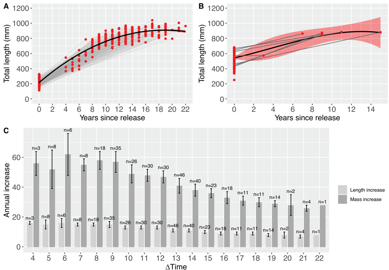
Fig. 2. Length differences between release and catch for PIT-tagged European eels ( Anguilla anguilla ) released in Lake Ymsen, Sweden, for A) released as small yellow eels (years 1998, 1999 and 2000), and B) released as larger yellow eels (year 1999). Total length for all eels when released is shown at year 0 (i.e., irrespective of actual release year) and recaptured as the number of years since release. For each individual that has been recaptured (PIT-tagged as small yellow n = 334 , larger yellow eels n = 7 ), a line (grey) is shown between length (mm) at release and recapture. The solid black line represents a locally estimated scatterplot smoothing (LOESS) curve, which models the relationship between years since release and total length (mm), with the red shaded region representing the 95% confidence interval for the estimated curve. Panel C shows mean ( \pm 1 SD) percentage increase in specific growth rates (SGR) for each year since release ( \Delta\text{Time} = \text{recapture date} - \text{release date} ), calculated based on mass ( \text{g year}^{-1} ) and length ( \text{mm year}^{-1} ), and the number of individuals ( n ) in each group. Only recaptured eels PIT-tagged as small yellow eels were included.
