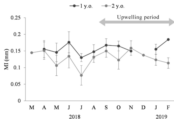
Fig. 4. Monthly means of marginal increment (MI) for 1 year (●) and 2 years-old (●) Auxis thazard landed in the Southeastern Brazil between March 2018 and February 2019. Vertical bars denote 95% confidence interval.
