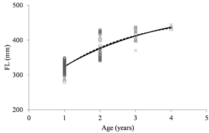
Fig. 7. von Bertalanffy growth curves for females (-----) and males (—) of Auxis thazard landed in Southeastern Brazil between March 2018 and February 2019. Symbols represent observed lengths for females (O) and males (x).
