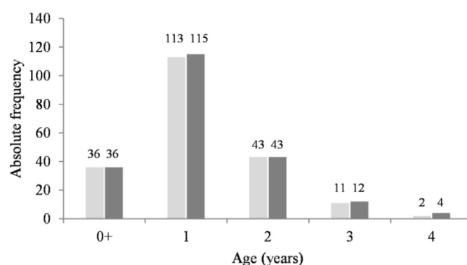
Fig. 6. Age composition of females (■) and males (■) of Auxis thazard landed in the Southeastern Brazil between March 2018 and February 2019. Numbers above bars correspond to number of aged fishes.
