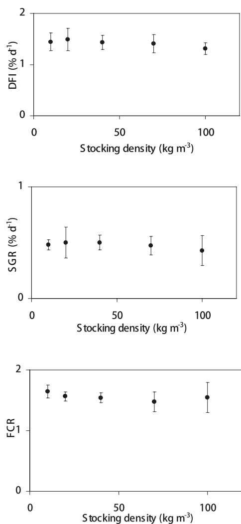
Fig. 1. Daily feed intake (DFI, % d -1 ), specific growth rate (SGR, % d -1 ) and feed conversion ratio (FCR) of sea bass reared at five density treatment (10, 20, 40, 70, 100 kg m -3 ) during the 84-day experiment. Statistical results are given, NS as non significant difference ( p > 0.05 ) between groups.
