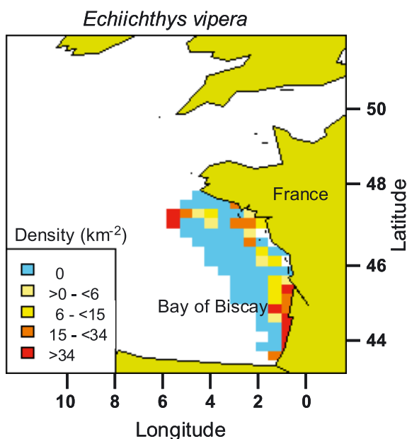
Fig. 2. Checking spatial coverage of survey data series. Average density per km 2 for lesser weever in the Western IBTS groundfish survey (1987-2006). Categories are quantiles.
