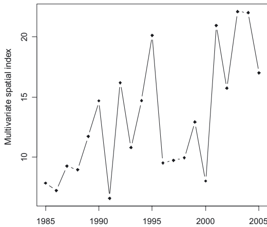
Fig. 3. Time series of the MFA-based multivariate spatial index D^2(t) . The index is a square distance in the MFA factorial subspace of the two first principal components measuring the departure in each year from the reference average spatial pattern over all age groups.
