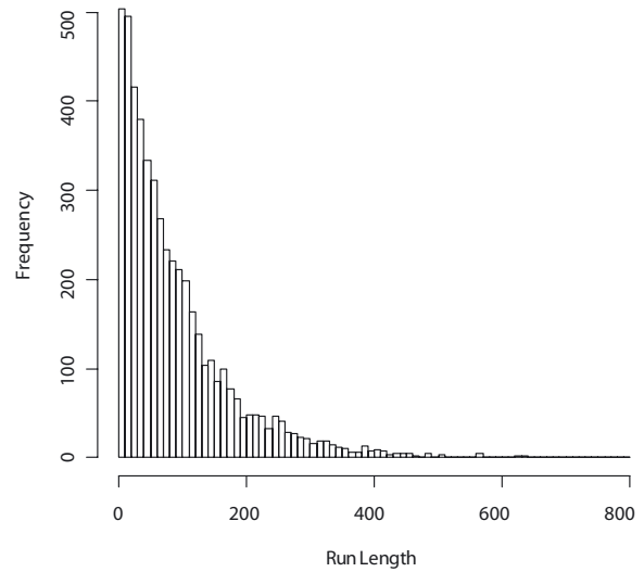
Fig. 4. Distribution of the (in-control) Run Length RL(0) of the CUSUM sequence for the multivariate spatial index D^2(t) that is \chi^2 with 10 degrees of freedom \chi^2(10,0) . The run length RL(0) is the time to a false alarm when no change in the distribution parameters has occurred.
