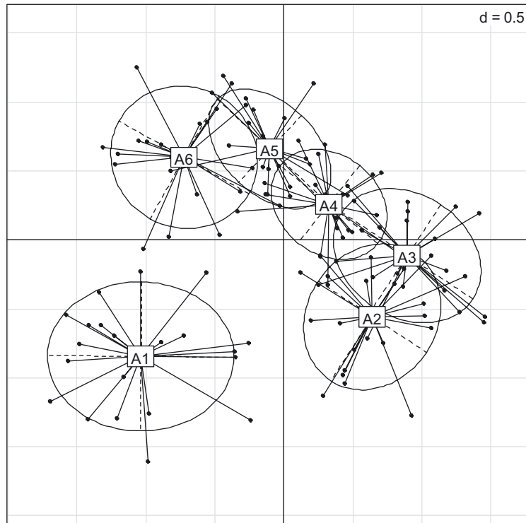
Fig. 1. MFA representation of the North Sea cod age-structured spatial pattern. The points represent the spatial distribution of each age in each year. The age labels represent the age-specific gravity centres, materialising the reference age-structured spatial pattern.
