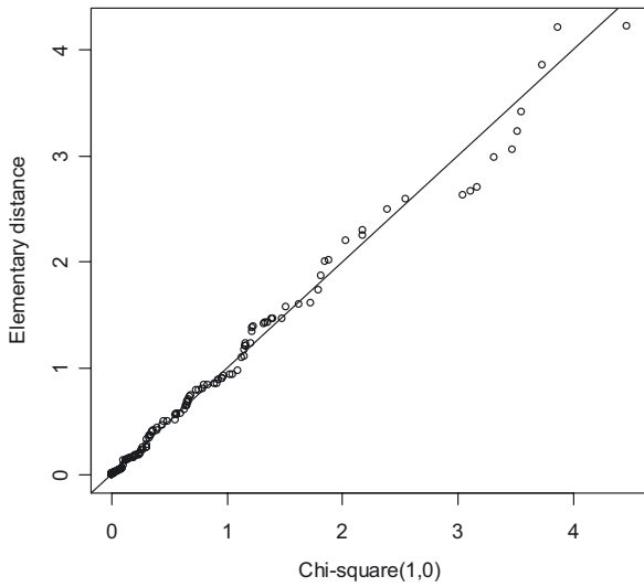
Fig. 2. Q-Q plot between the elementary square distances d_{k,a,t}^2 and the \chi^2 distribution with one degree of freedom, for the reference period (1985-1994).
