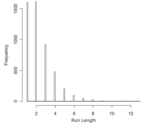
Fig. 5. Distribution of the (out-of-control) Run Length RL(ncp) of the CUSUM sequence for the multivariate spatial index D^2(t) that is \chi^2 with 10 degrees of freedom \chi^2(10,0) . The run length RL(ncp) is the time to detect a change in the non centrality parameter ncp when it has effectively happened.
