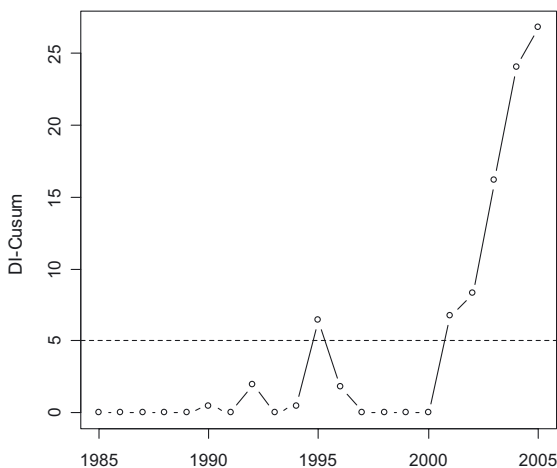
Fig. 6. Decision-interval CUSUM (DI-CUSUM) control chart for monitoring the multivariate spatial indicator D^2(t) . The in-control distribution of the indicator is a \chi^2 with 10 degrees of freedom \chi^2(10, 0) . The values above the threshold indicate an out-of-control state in which the non centrality parameter has shifted from 0 to 11. The detection is achieved with an average false alarm rate of 0.04 and an alarm detection time of 2 years. The parameters of the CUSUM scheme are ck = 14.2 (allowance) and ch = 5 (decision interval).
