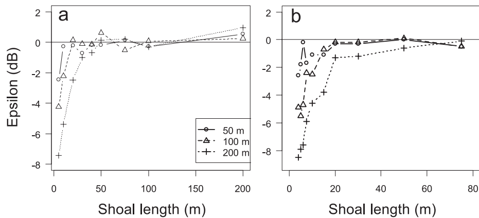
Fig. 6. Impact of horizontal dimension and density on measurement bias \varepsilon = 10 \log_{10}(\hat{\sigma}_{ag}) - 10 \log_{10}(\sigma_{ag}) as a function of shoal length at different depths (50, 100 and 200 m); a) scenario 1 for a single shoal with variable horizontal dimensions; b) scenario 2 for groups of shoals with different horizontal dimensions but same density and overall same total number of individuals.
