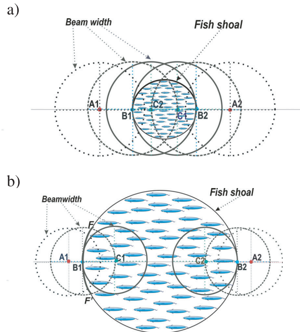
Fig. 2. Diagram in horizontal plane of the process of a shoal detection by a vertical echosounder. a) shoal size is smaller than the beam; b) shoal size is larger than the beam.
