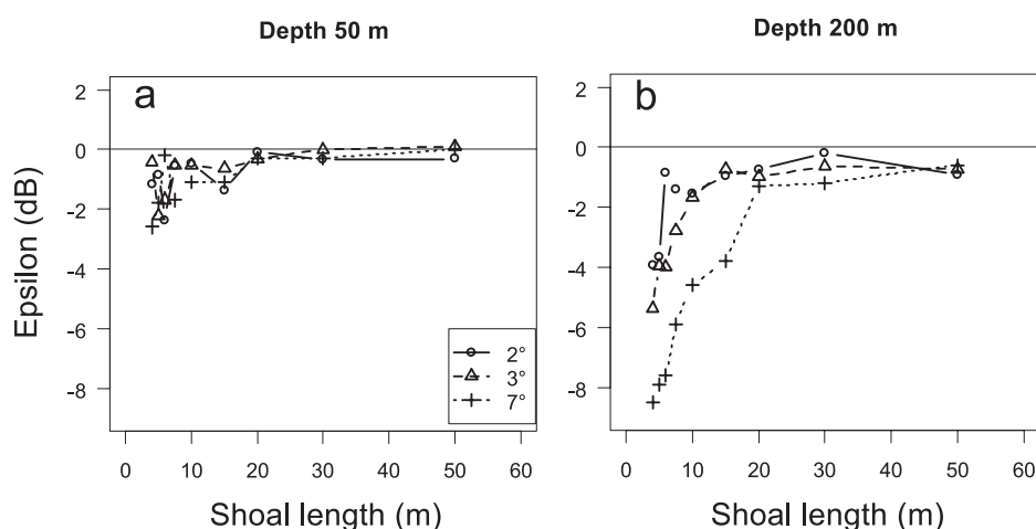
Fig. 7. Impact of beam width on measurement bias \varepsilon = 10 \log \hat{\sigma}_{ag} - 10 \log \sigma_{ag} as a function of shoal length. Results from scenarios 2 and 3 at a) 50 m, b) 200 m.
