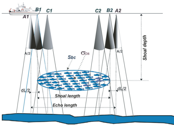
Fig. 1. Diagram in vertical plane of the process of shoal detection by a vertical echosounder.
