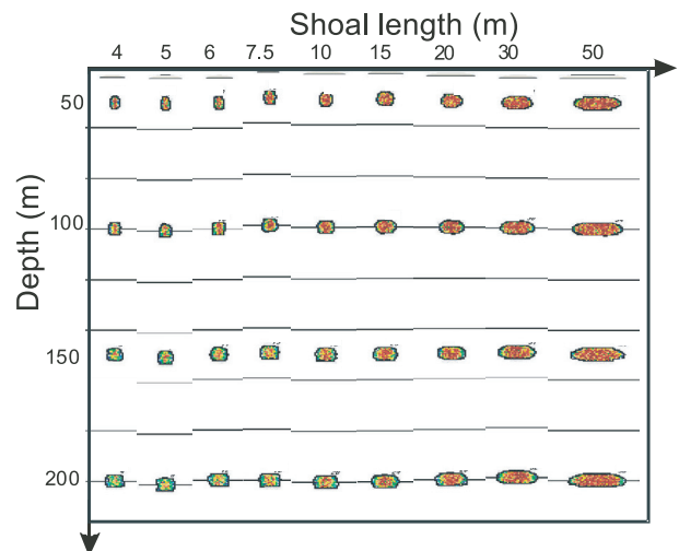
Fig. 5. Echograms of simulated shoals for scenario 3 for 3° beam width.
