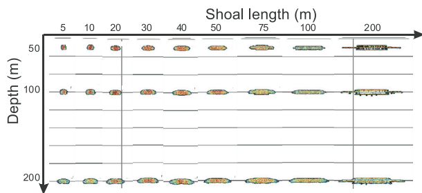
Fig. 3. Echograms of simulated shoals for scenario 1.
