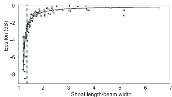
Fig. 8. Measurement bias \varepsilon = 10 \log_{10}(\hat{\sigma}_{ag}) - 10 \log_{10}(\sigma_{ag}) as a function of shoal size relative to beam width based on simulations for scenario 4. The vertical line indicates the limit value of 1.3 below which no bias correction is possible.
