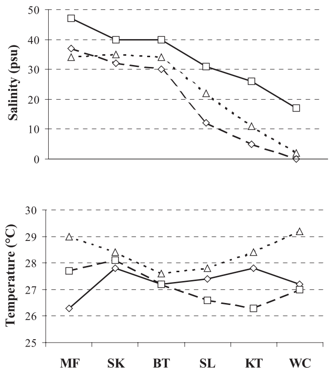
Fig. 2. Spatial and temporal variation of environmental parameters in Gambia estuary during 2002: a) salinity; b) temperature. (solid line = May; small dotted line = September; large dotted line = November).
