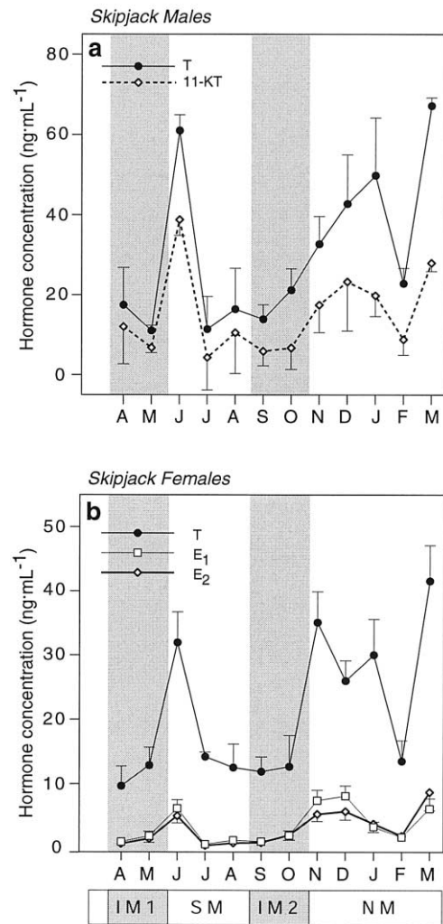
Figure 4. Monthly variations of testosterone (T) and 11-ketotestosterone (11-KT) in skipjack tuna males (a) and T, oestrone (E 1 ) and oestradiol (E 2 ) in skipjack tuna females (b). IM1: intermonsoon 1, SM: south monsoon, IM2: intermonsoon 2, NM: north monsoon. Vertical bars indicate the standard error of the mean. Number of fish sampled as in figure 2.
