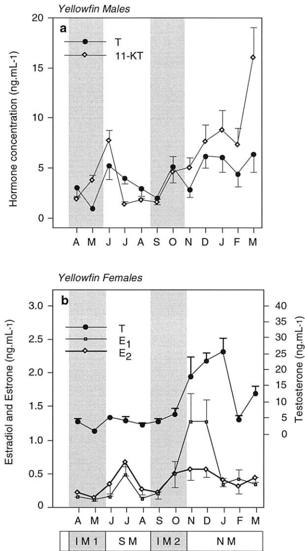
Figure 3. Monthly variations of testosterone (T) and 11-ketotestosterone (11-KT) in yellowfin tuna males (a) and T, oestrone (E 1 ) and oestradiol (E 2 ) in yellowfin tuna females (b). IM1: intermonsoon 1, SM: south monsoon, IM2: intermonsoon 2, NM: north monsoon. Vertical bars indicate the standard error of the mean. Number of fish sampled as in figure 2.
