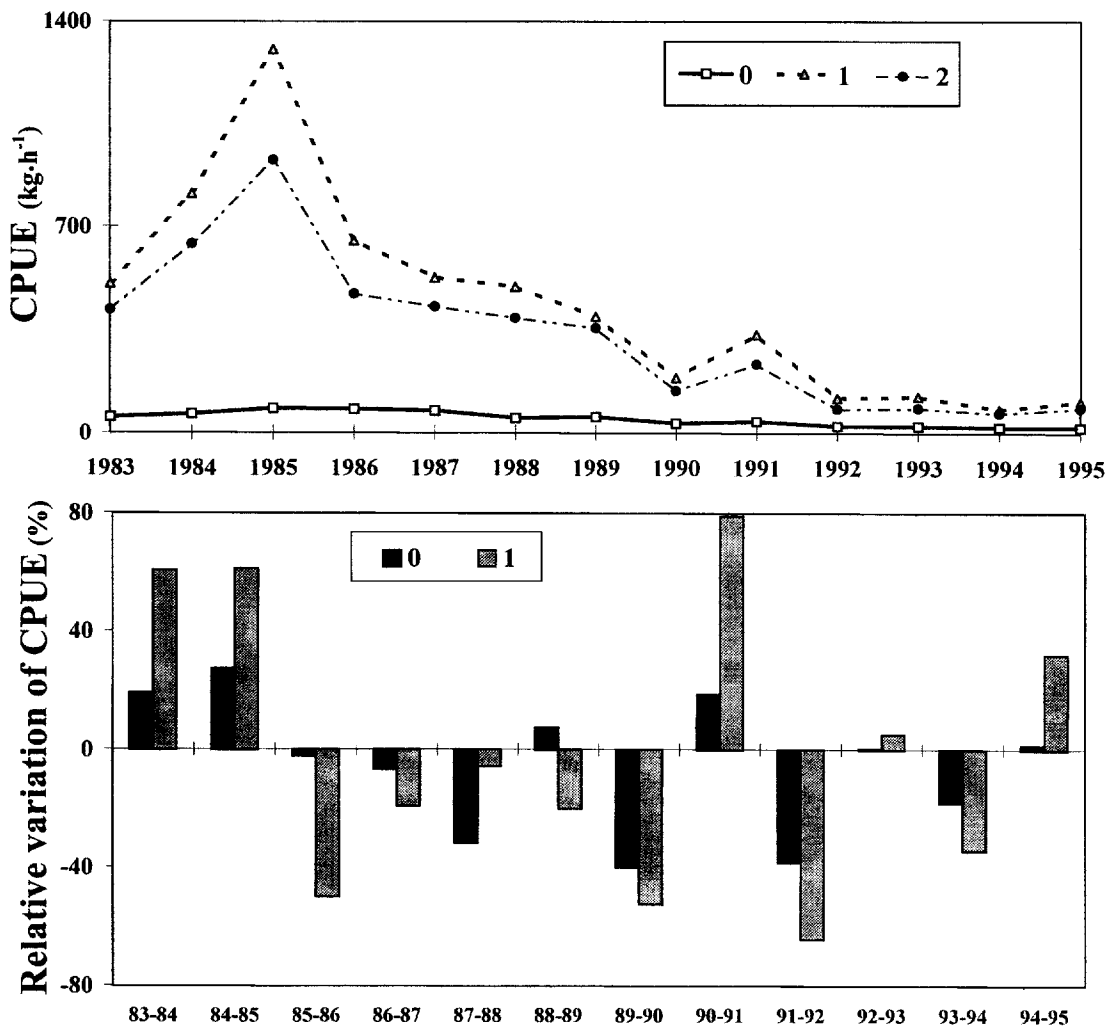
Figure 9. Blue ling (west coast of Scotland). Trends of French CPUE and relative variations for global and directed series: 0 = Global CPUE, i.e., Total landings / Total effort in sub-area VI (fishing time); 1 = blue ling métier (pure métier defined from 75 % EQL); 2 = blue ling métier (pure métier defined from 90 % EQL).
