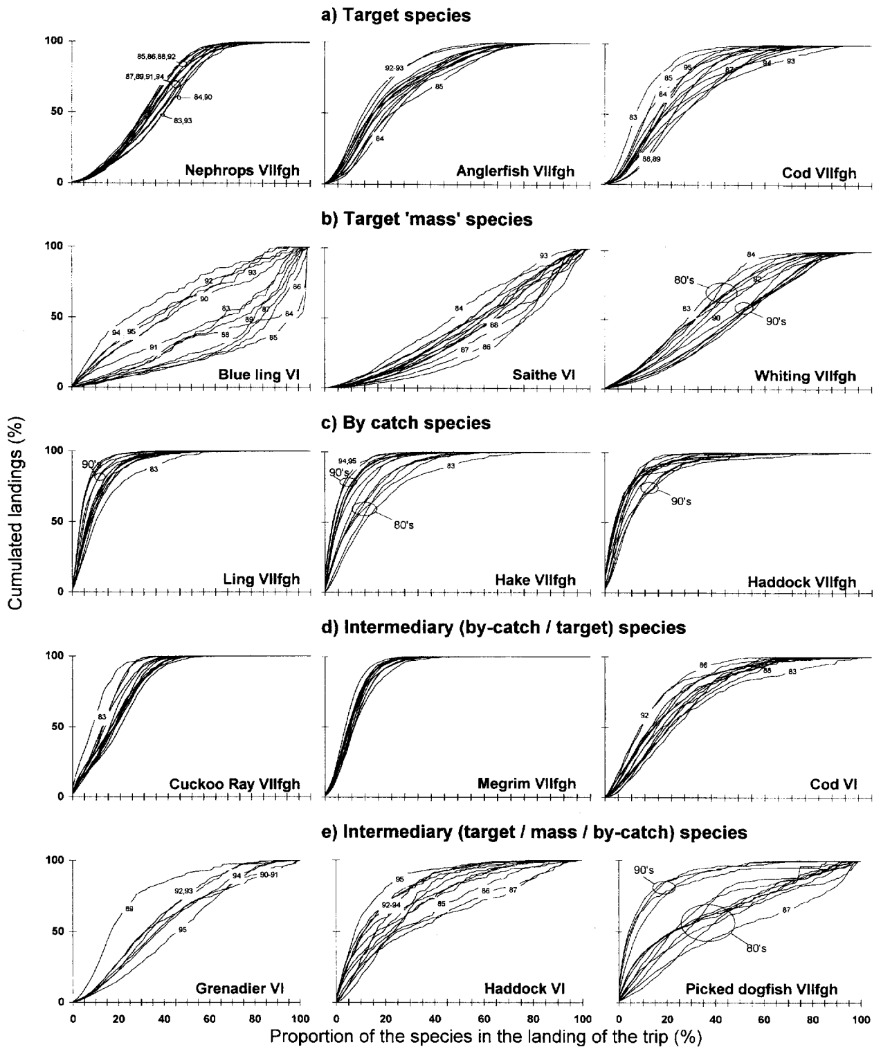
Figure 2. Cumulative relative landings of the French demersal fishery off the west coast of Scotland (ICES sub-area VI) and in the Celtic Sea (ICES divisions VII fgh) for some (a) Target species, (b) Target 'mass' species, (c) By-catch species, (d) and (e) Intermediary species. X-axis is the percentage of each species (in weight) in the landings of each fishing trip (truncated value). Y-axis is the cumulated percentage of landings for trips for which the species represents less than the given (in abscissa) in the fishing trip landings.
