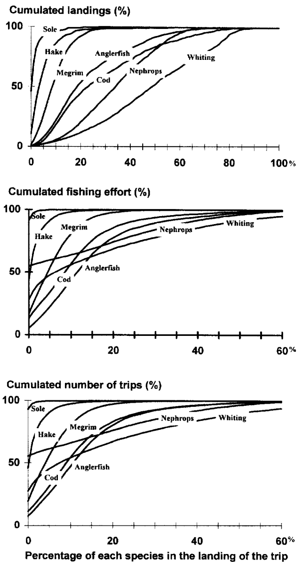
Figure 1. Example of three types of graph showing: (a) the cumulative relative landings; (b) the cumulative relative fishing effort; (c) the cumulative number of fishing trips. X-axis is the percentage of each species (in weight) in the landings of each fishing trip (truncated value). Y-axis is the cumulated percentage of landings, effort or number of trips, for trips for which the species represents less than the given (in abscissa) in the fishing trip landings.
