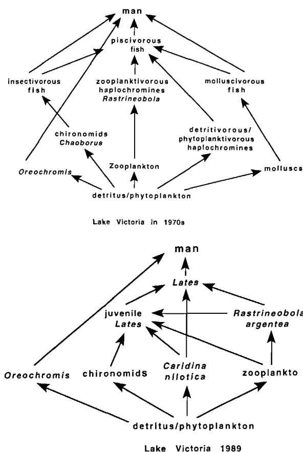
Figure 4. – Simplified diagrams of the food web in the sub-littoral area (6-20 m deep) of Lake Victoria in the 1970s and in 1989 (Modified from Ligotvoet and Witte, 1991).
