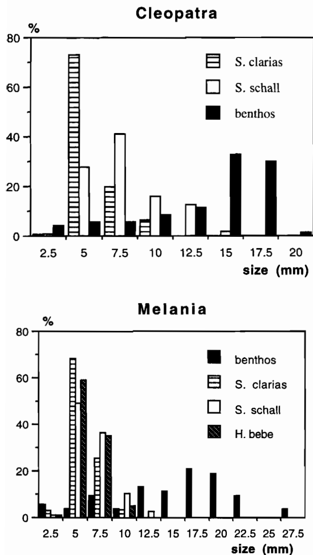
Figure 1. – Comparison of size distribution of benthic molluscs in Lake Chad benthos and in the gut of malacophagous fish species ( Synodontis clarias , S. schall , Hyperopisus bebe ) (data from Lauzanne, 1975).
