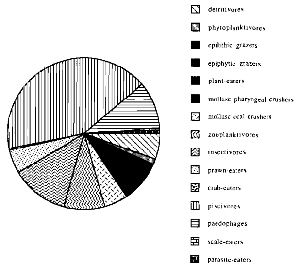
Figure 8. – Trophic specialisations among Cichlids in Lake Victoria and relative number of species (data from Witte and van Oijen, 1990).
