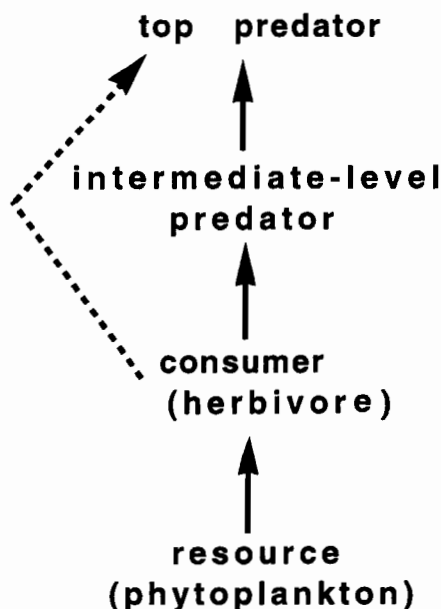
Figure 6. – The geometry of a cascading trophic interaction with and without intraguild predation. Trophic cascades are only possible if the IGP link is not strong compared to the link between the top and intermediate-level predators (from Polis and Holt, 1992).
